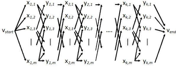
Figure 1: Reformulation of mb-TTP as a shortest path problem.
