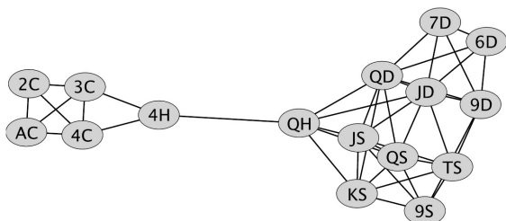
Figure 2: The match-by-card graph of the deal in Table 11.
