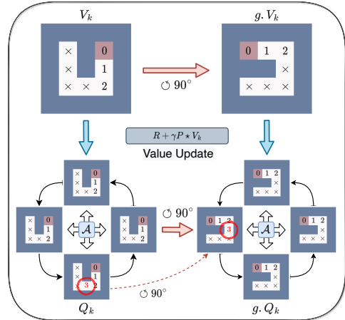
Figure 4: Commutative diagram of a single step of value update, showing equivariance under rotations. Each grid in the Q -value field corresponds to all the values Q(\cdot, a) of a single action a .
