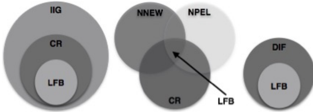
Fig. 2. Visual representation of relationships among the sets of ranking relations
