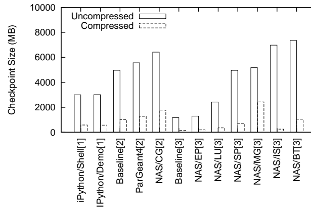
(c) Aggregate (cluster-wide) checkpoint size.
