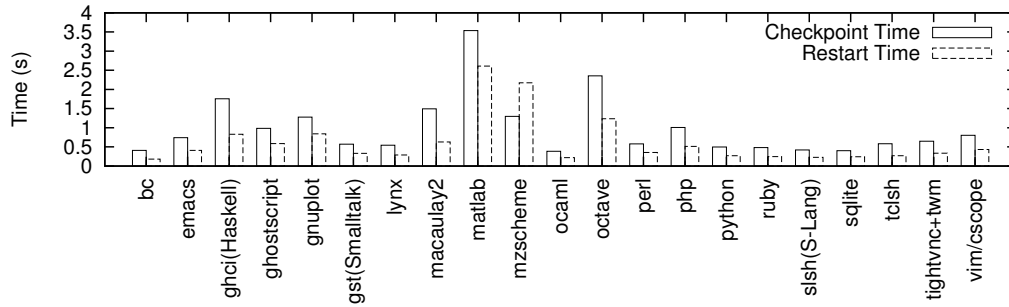
(a) Checkpoint/Restart timings.
