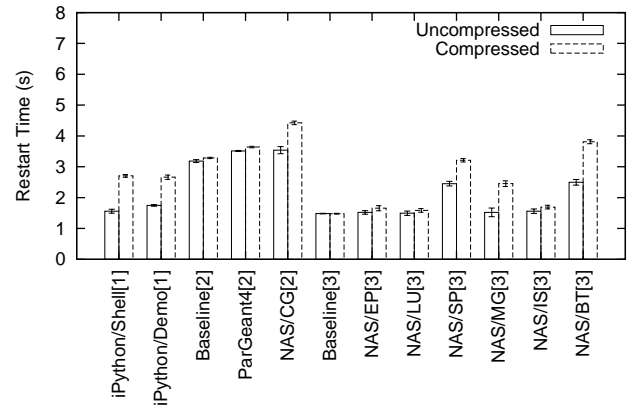
(b) Restart timings.
