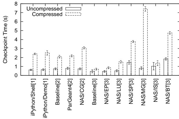
(a) Checkpoint timings.
