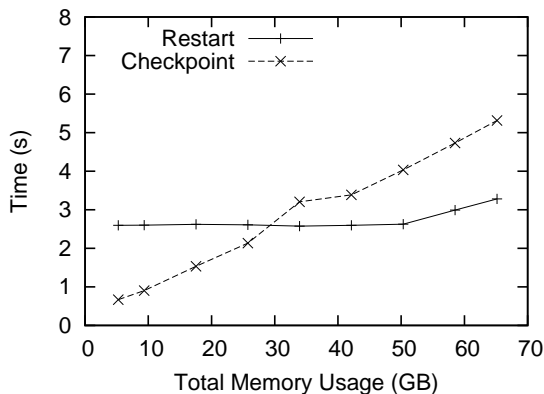
Figure 6: Timings as memory usage grows. A synthetic OpenMPI program allocating random data on 32 nodes. Compression is disabled. Checkpoints written to local disk.
