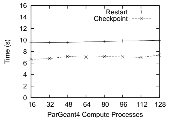
(b) Checkpoints stored to centralized RAID storage via SAN and NFS.
